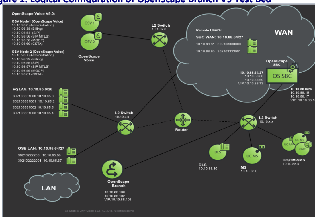
Figure 1: Logical Configuration of OpenScape Branch V9 Test Bed
